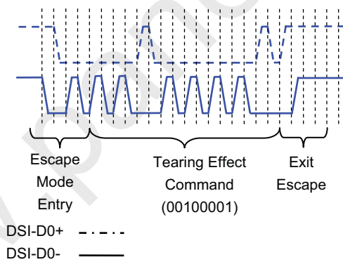
Figure 9 Acknowledge Trigger.
