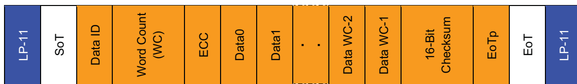
Figure 15 Long Packet Format.
