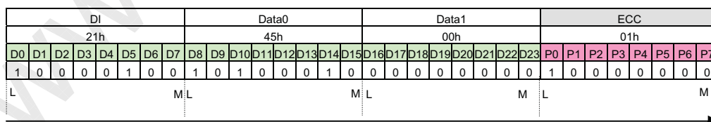
Figure 34 DCS Read Short Response, 1 byte Returned.
