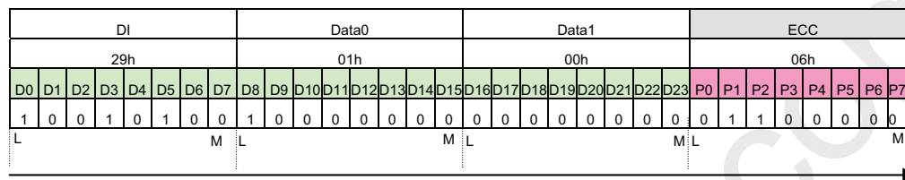
Figure 19 Error Correction Code on the Short Packet.
