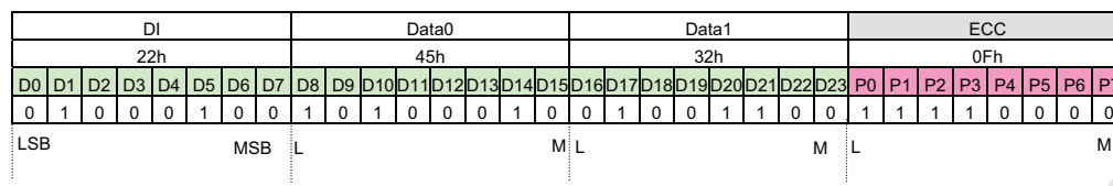
Figure 35 DCS Read Short Response, 2 bytes Returned.
