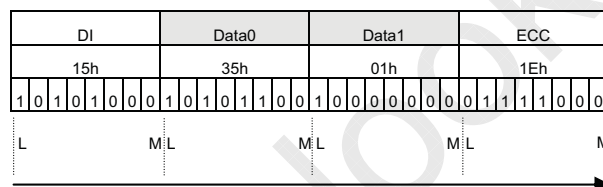
Figure 17 Data on the Short Packet.
