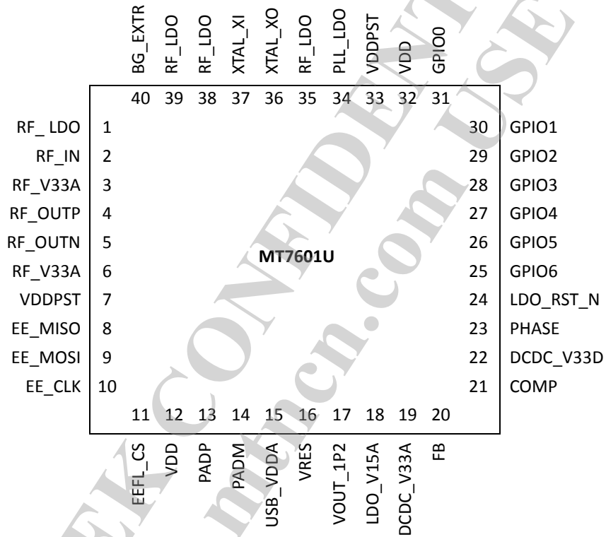
Figure 2 Top view of MT7601U QFN pin-out.
