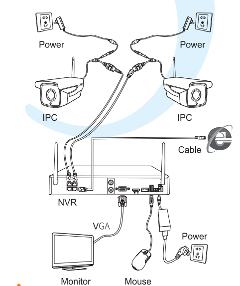
Wired connection diagram
