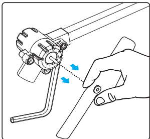
3.2 Hold the middle of the tail rotor and remove both ends of it
